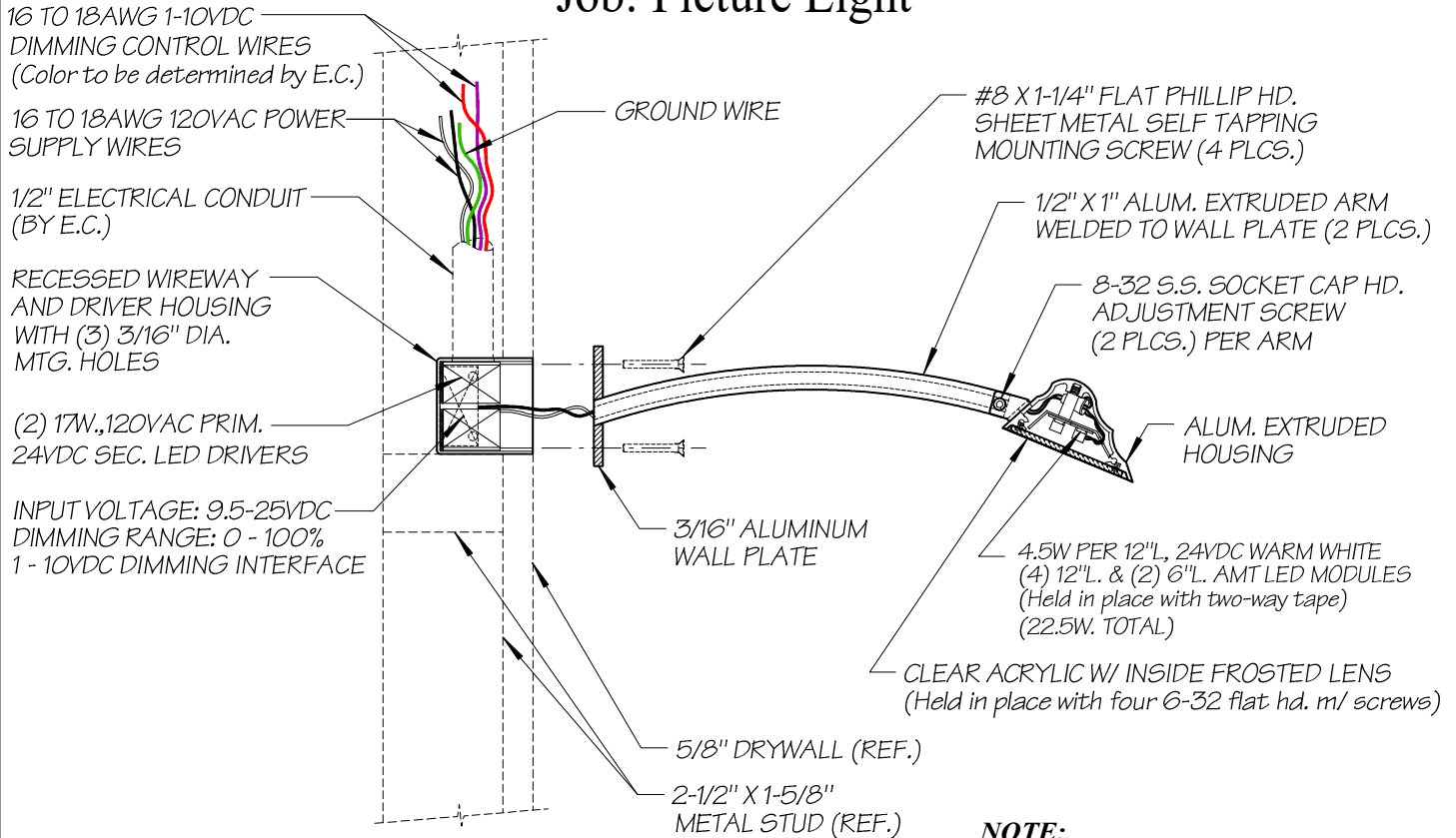
SIDE / SECTION VIEW
